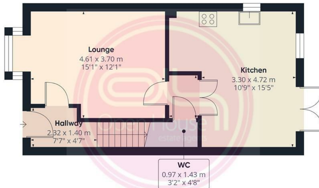
Floor 0
